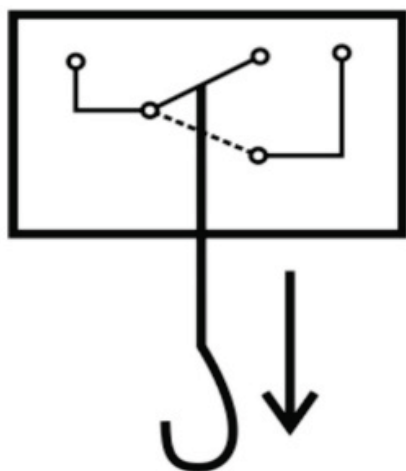
Figure 3-5 Detector of a painting, schematic illustration
